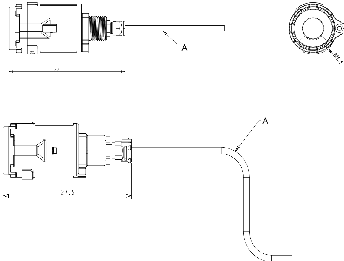
Figure 1 : Dimensions
